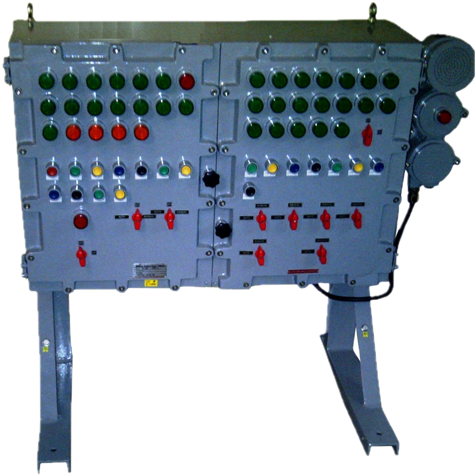
STAND ALONE TYPE JUNCTION BOX NJB 40550
